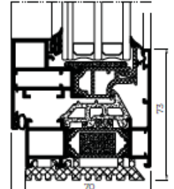
HIDDEN DRAINAGE
