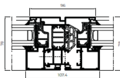
FLOATING MULLION
